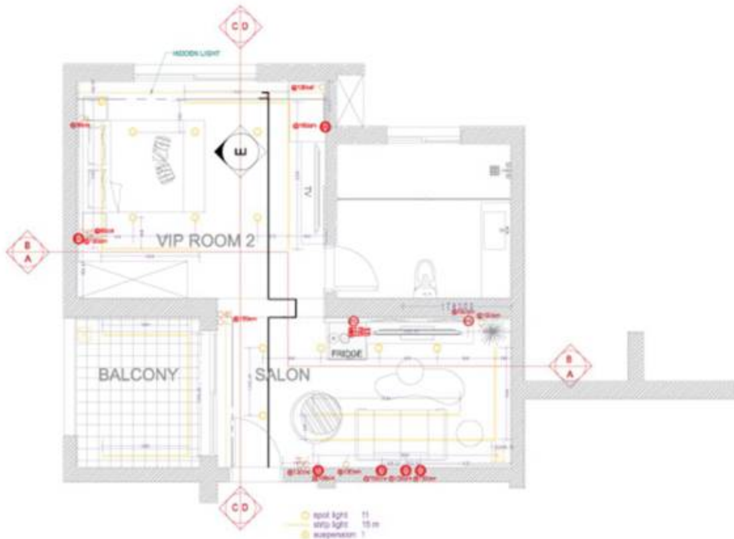
Lighting & Electrical Plan
