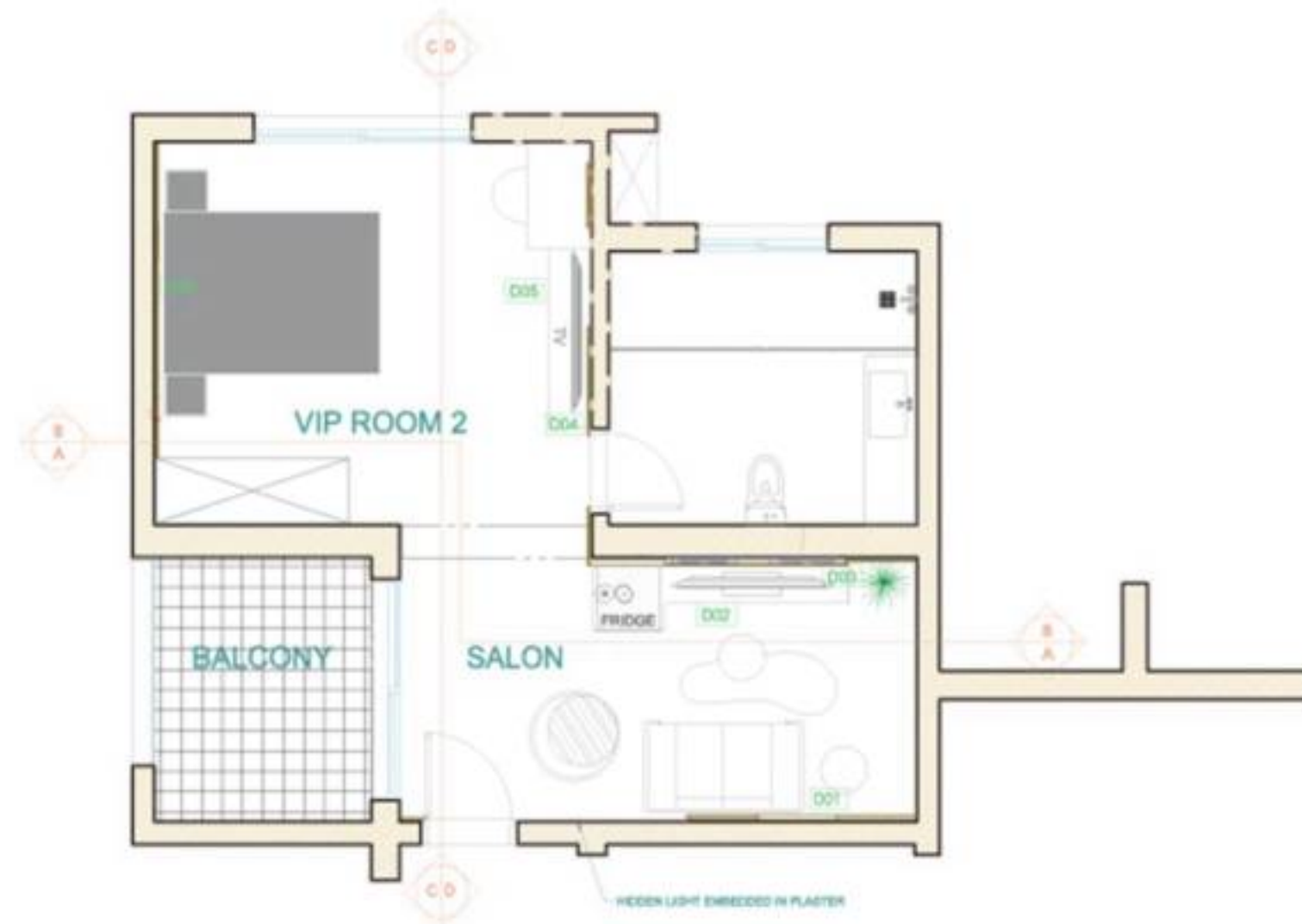
Suite Furniture Layout
